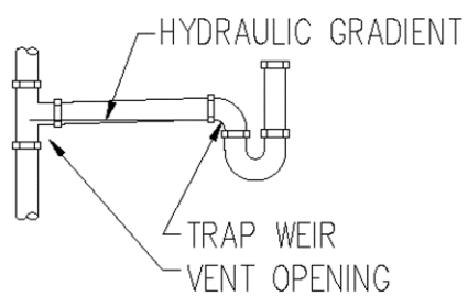
SATISFACTORY INSTALLATION
