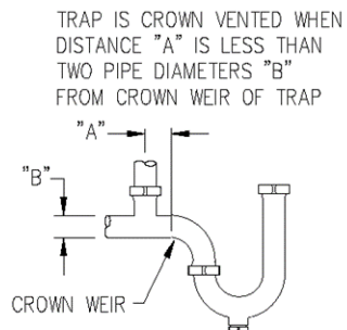
CROWN VENTED TRAP
