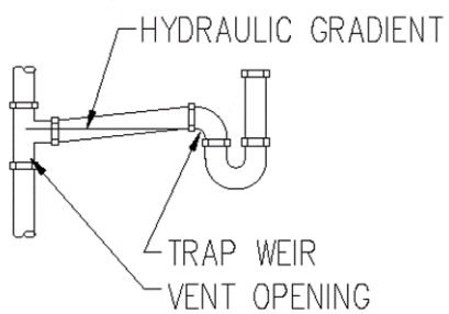
UNSATISFACTORY INSTALLATION
