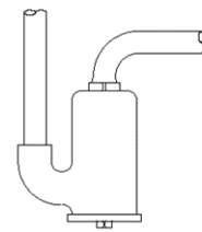
ANTI-SIPHON TRAP
